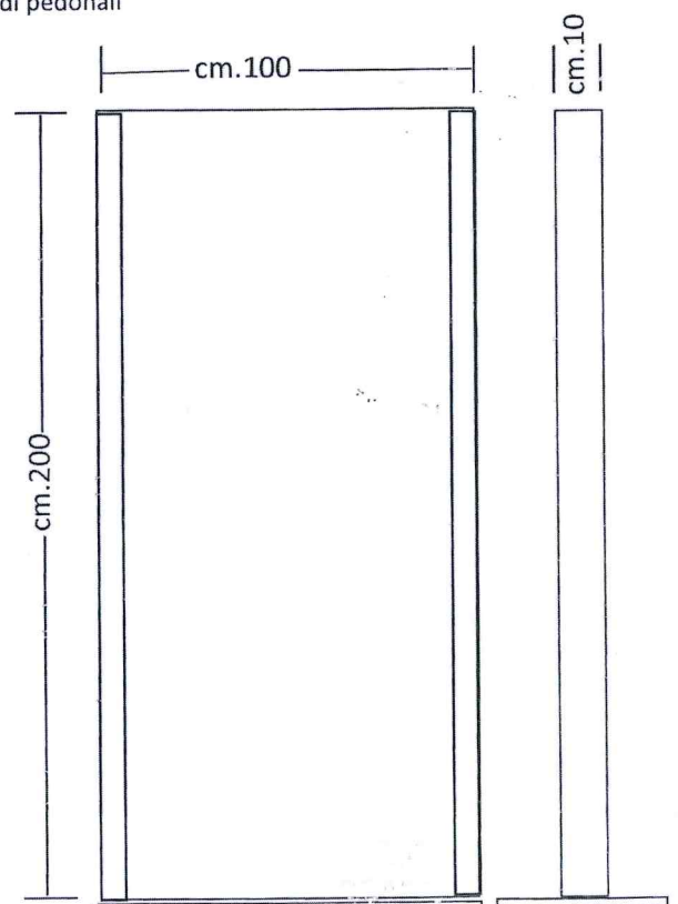
MISURE MINI-TOTEM
